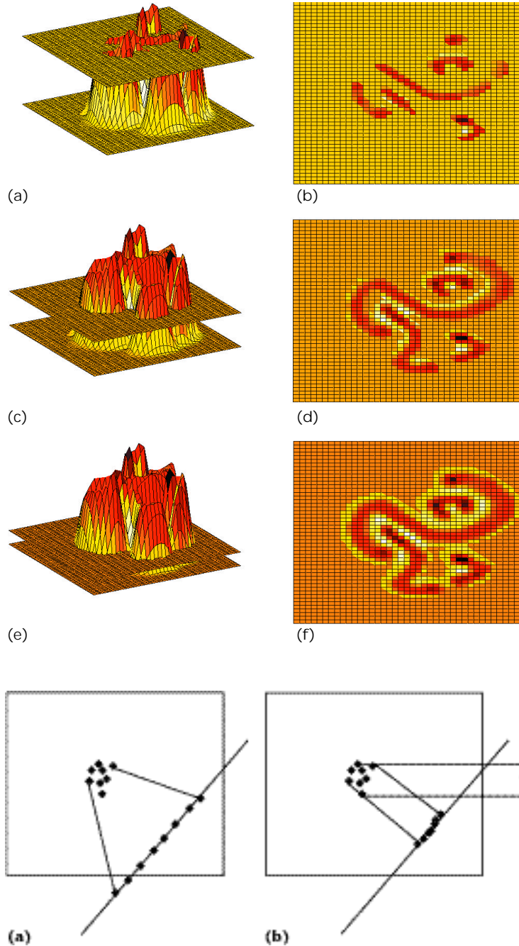
2 Example of multicenter-defined clusters for different \xi . (a), (b) \xi = 4 ; (c), (d) \xi = 2 ; and (e), (f) \xi = 1 .
