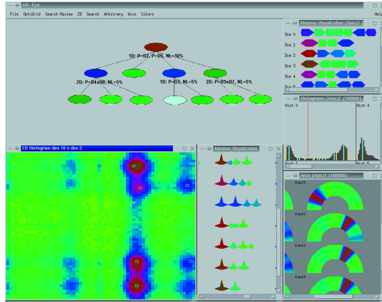
5 Examples of a projection and separator tree. Clockwise from the top: a projection and separator tree, iconic representation for 1D projections, curve-based density plots, color-based density plots, iconic representation for 2D projections, and a color-based 2D density plot.
